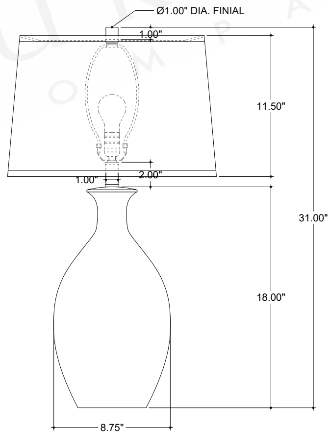
FRONT VIEW
