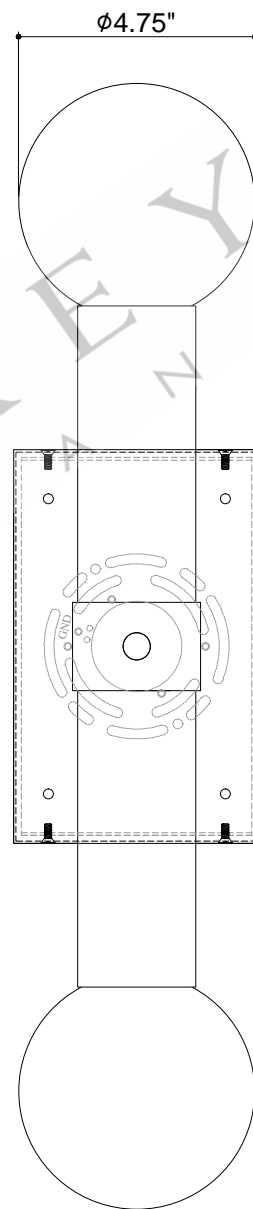
FRONT VIEW
