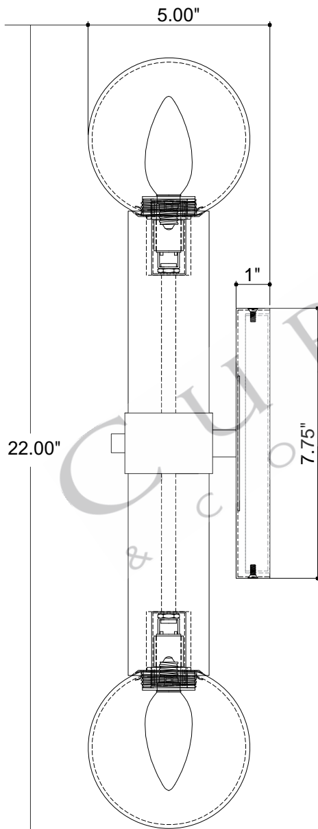
SIDE VIEW
