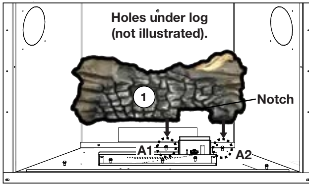
1. Place the holes in log #1 on A1 and A2. Ensure the notch fits around the pilot shield.
