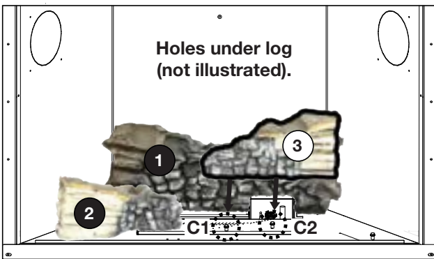
3. Place the holes in log #3 on C1 and C2. Do not cover any burner ports.
