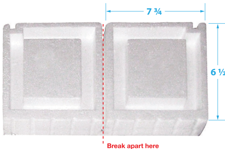
DVBP - 6 ½ in. x 16 in. Foundation Vents
