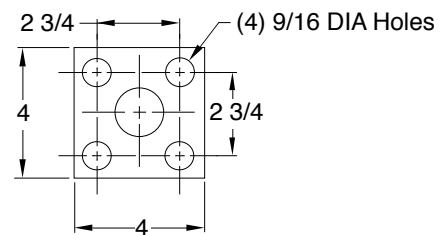
BASE DETAIL
