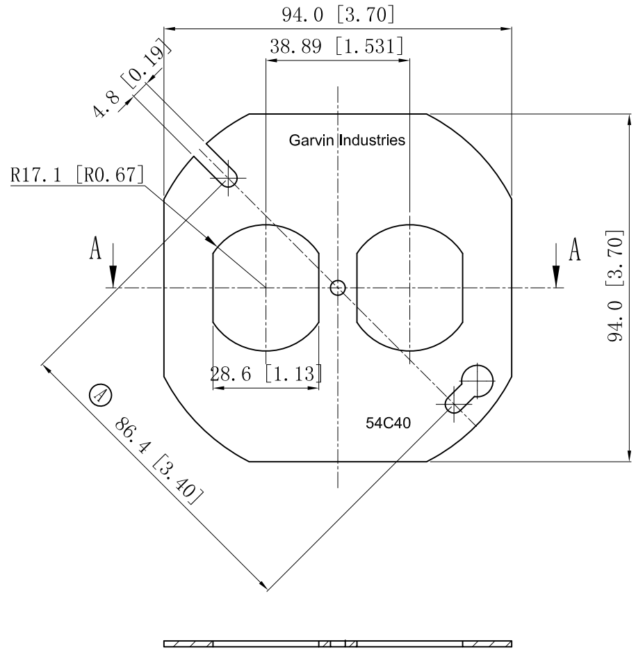
CUTAWAY VIEW A-A
