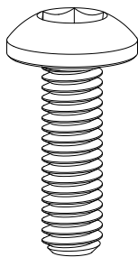
ALLEN KEY SCREW M6*20mm QTY 16
