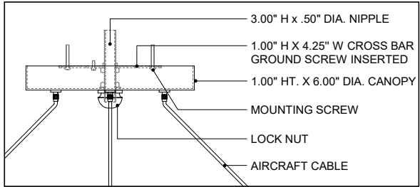
CANOPY DETAIL
