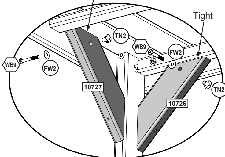
Inside and Underneath View
