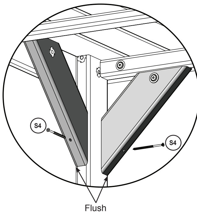
Inside and Underneath View
