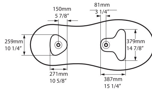
Underside view
