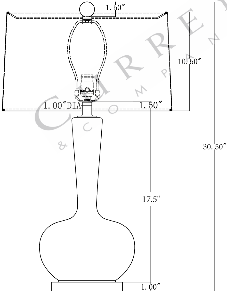
FRONT VIEW
