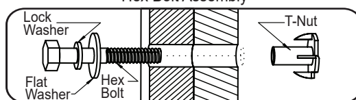
Hex Bolt Assembly
