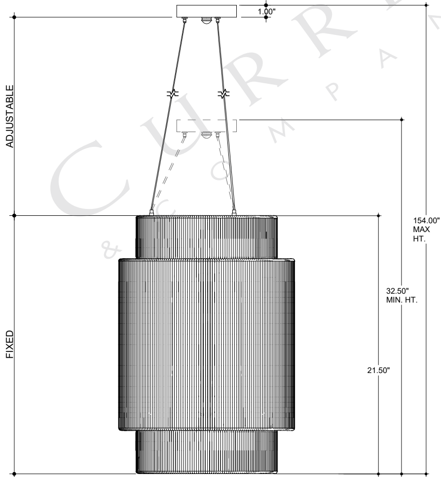
FRONT VIEW
