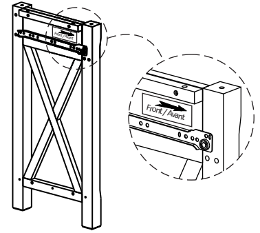
RIGHT SIDE QTY 1
