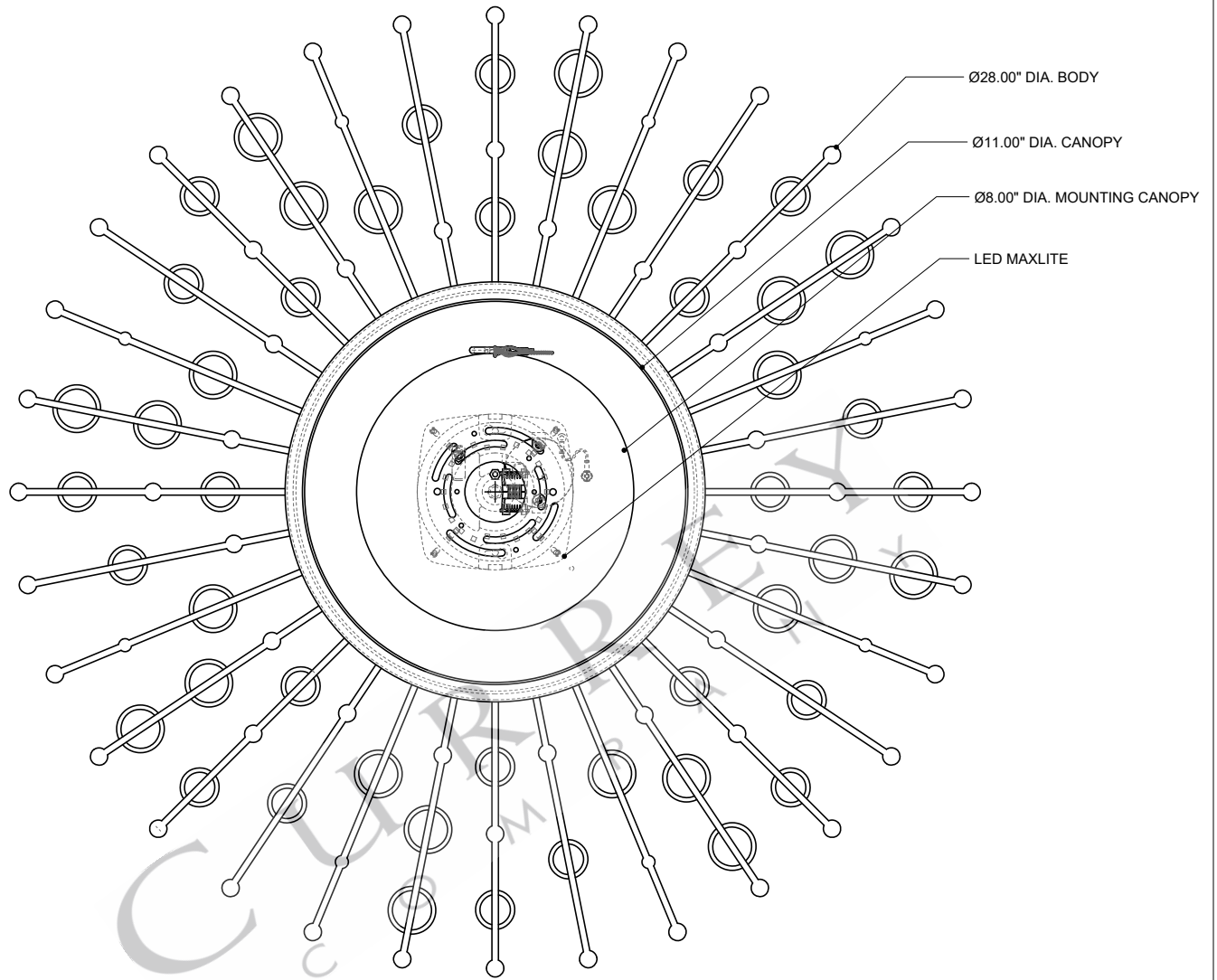
TOP VIEW
