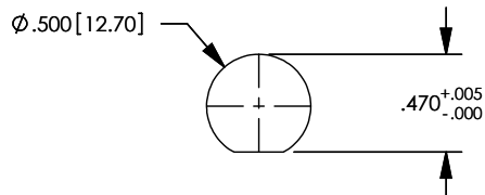
MOUNTING HOLE
