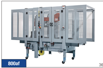
800af 36 3M-Matic™ Case Sealer 800af is an adjustable fully automatic case sealer.
