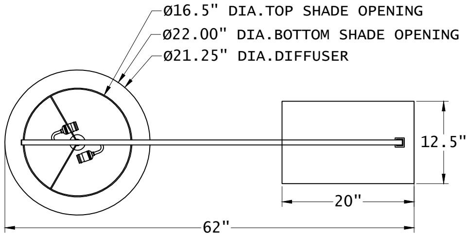
TOP VIEW
