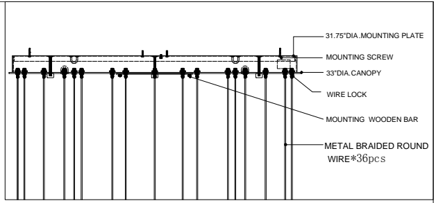
CANOPY DETAIL
