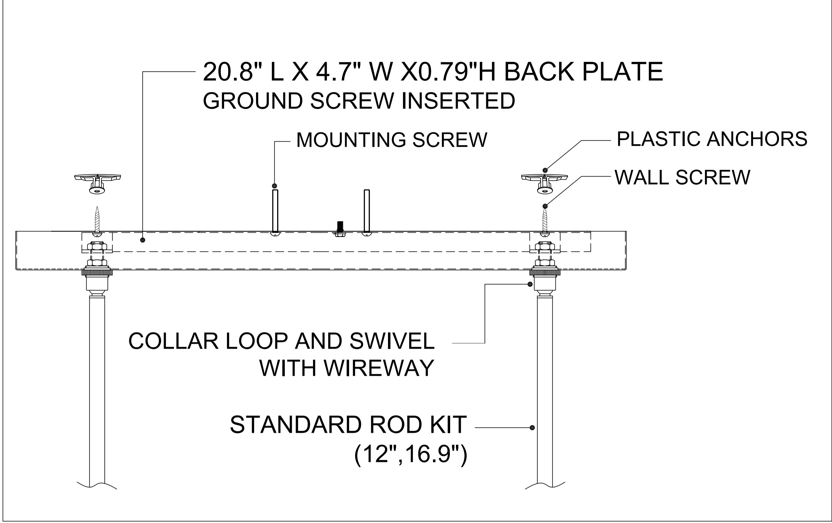
CANOPY DETAIL
