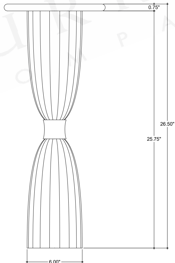
FRONT VIEW
