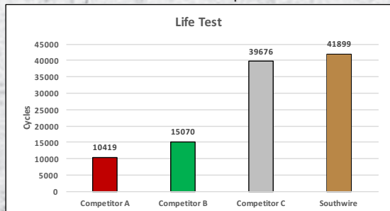
Life Number of Compressions
