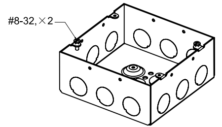
WELDING STYLE DETAIL VIEW B
