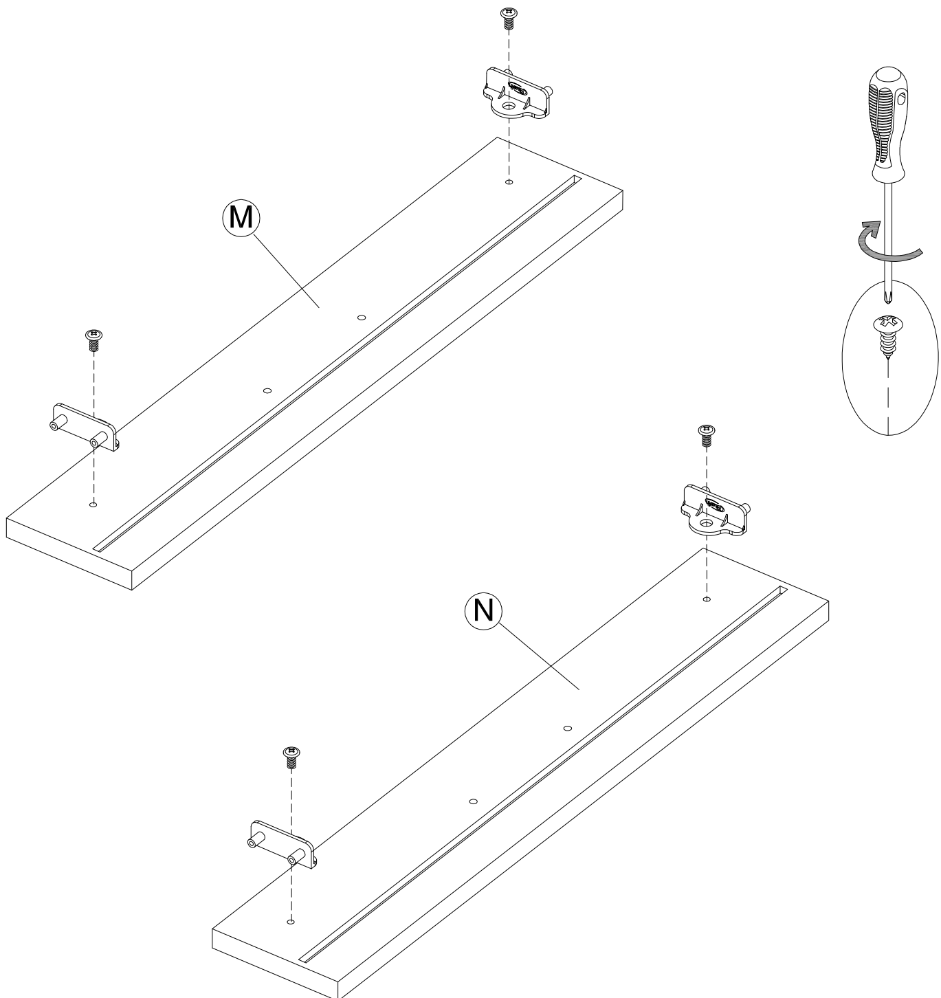
Drawer Bracket
