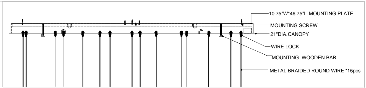
CANOPY DETAIL
