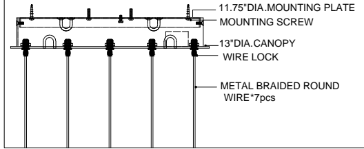
CANOPY DETAIL
