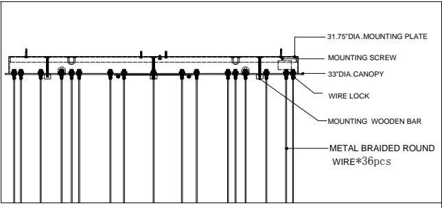
CANOPY DETAIL
