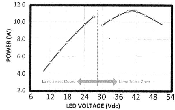
Figure 1 OUTPUT POWER
