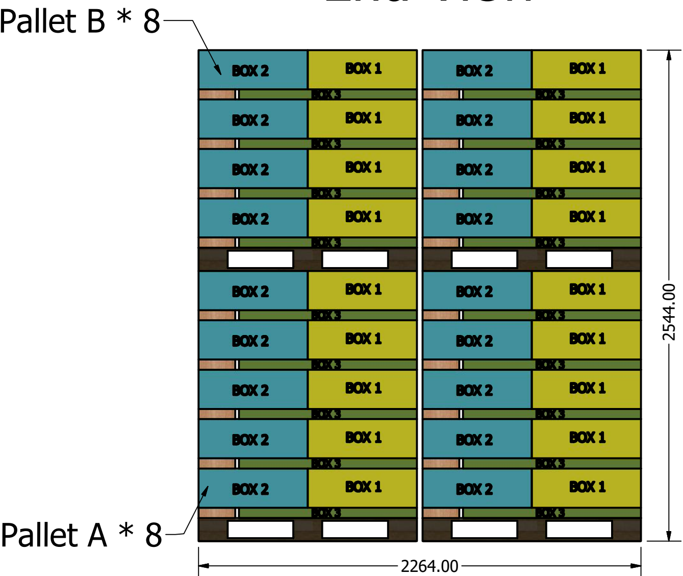
End View
