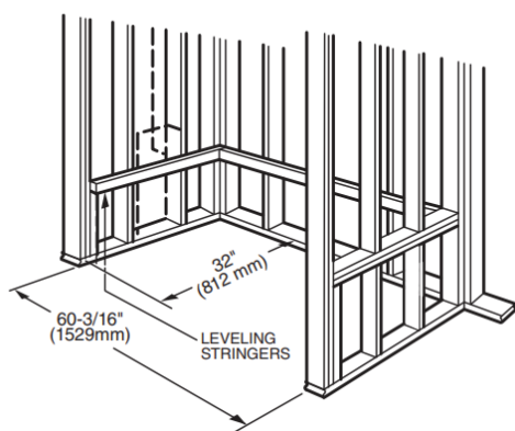
Typical Recess Installation
