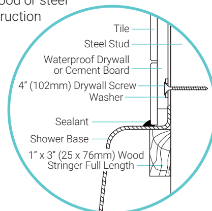
Steel Studs
