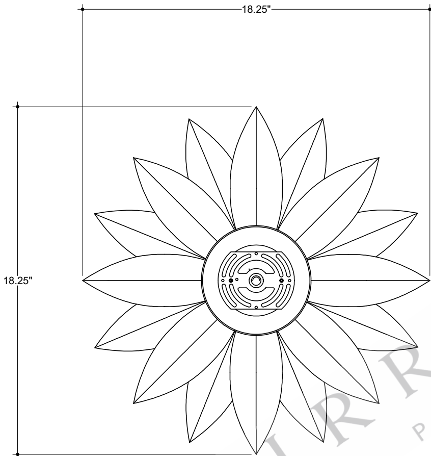
TOP VIEW
