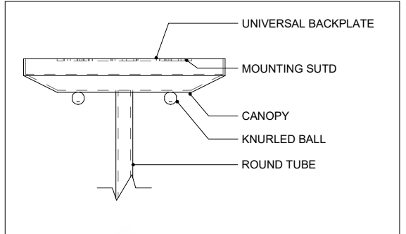
CANOPY DETAIL
