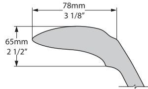
Rim detail
