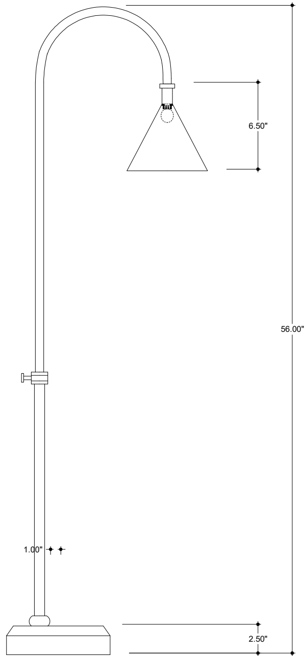
FRONT VIEW
