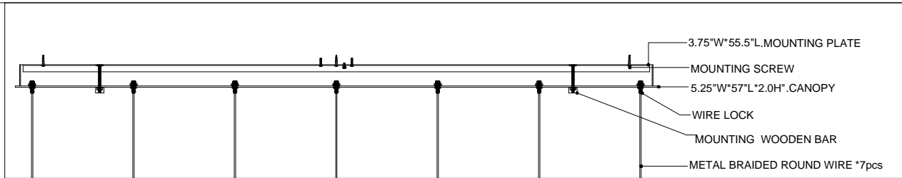
CANOPY DETAIL
