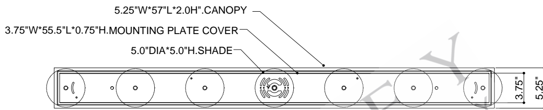
TOP VIEW
