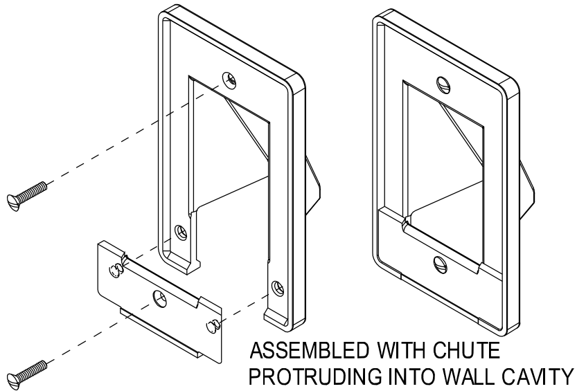
ISOMETRIC VIEWS
