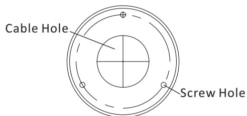
Figure 2-5 The Drill Template
