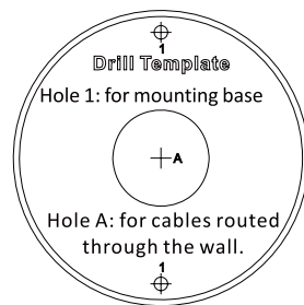
Figure 2-4 The Drill Template
