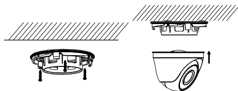
Figure 2-6 Fix the Mounting Base and Camera
