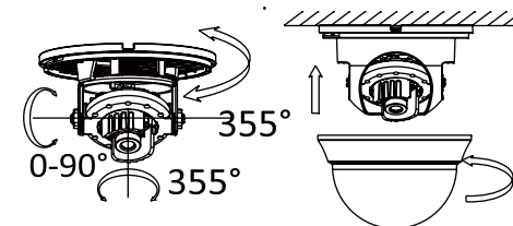
Figure 2-8 3-axis Adjustment & Lower Dome
