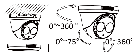
Figure 2-6 3-axis Adjustment
