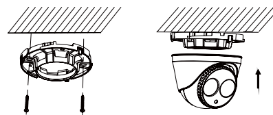
Figure 2-5 Fix the Mounting Base and Camera
