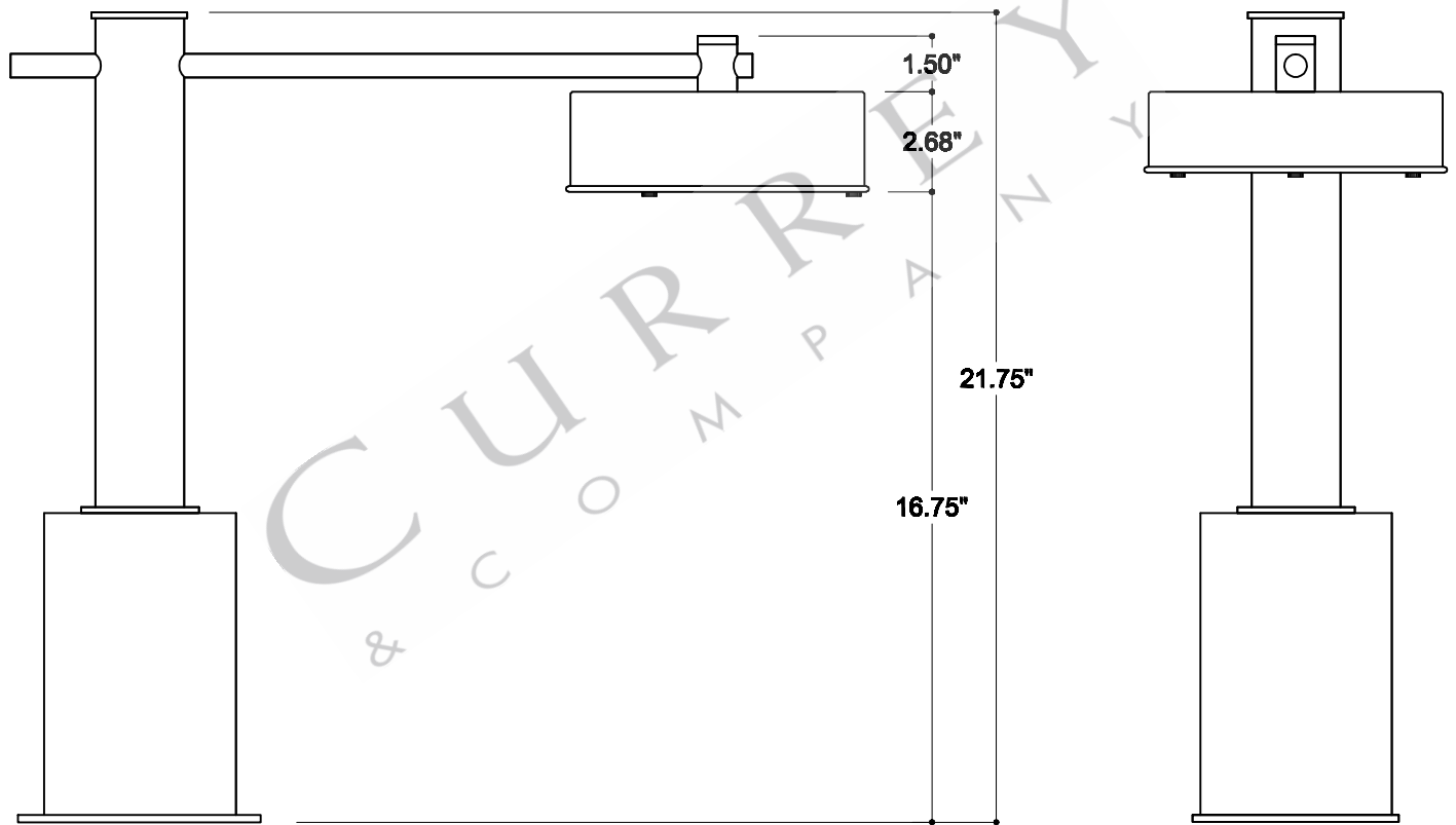
SIDE VIEW
