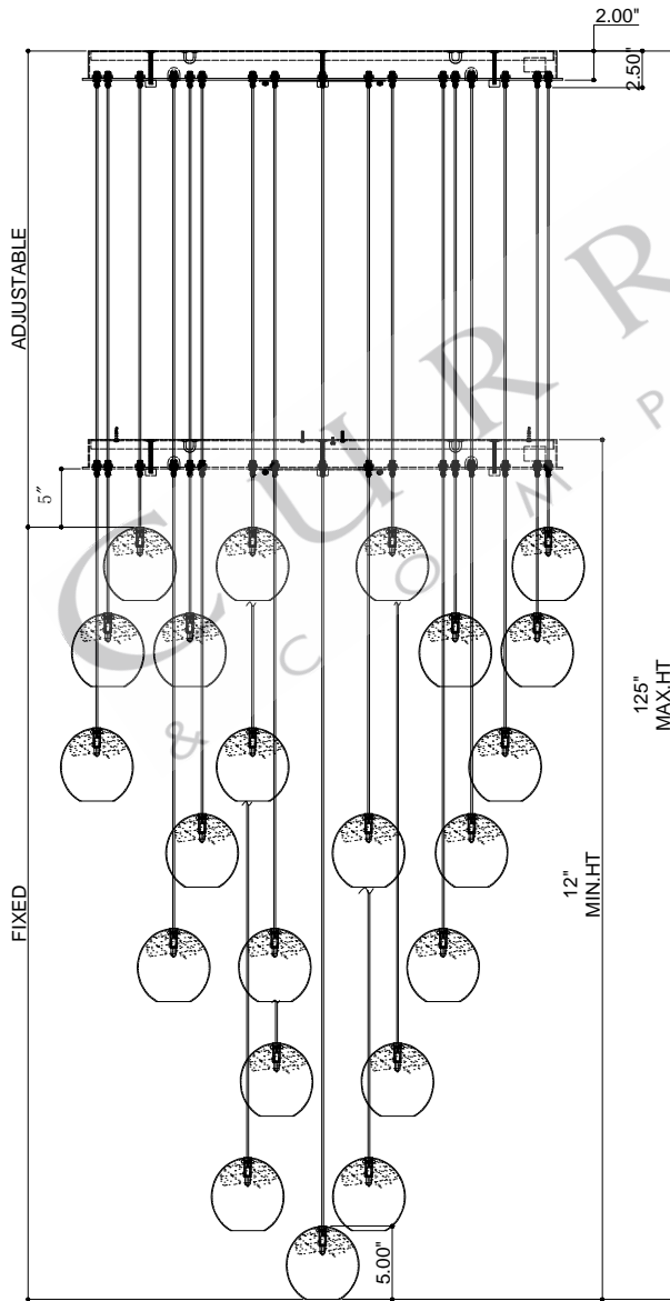
FRONT VIEW
