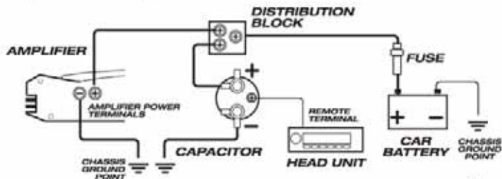
SUGGESTED WIRING
