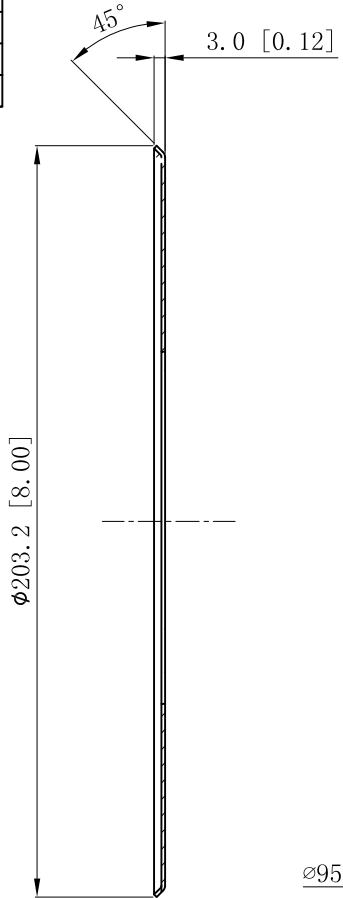
CUTAWAY VIEW A-A
