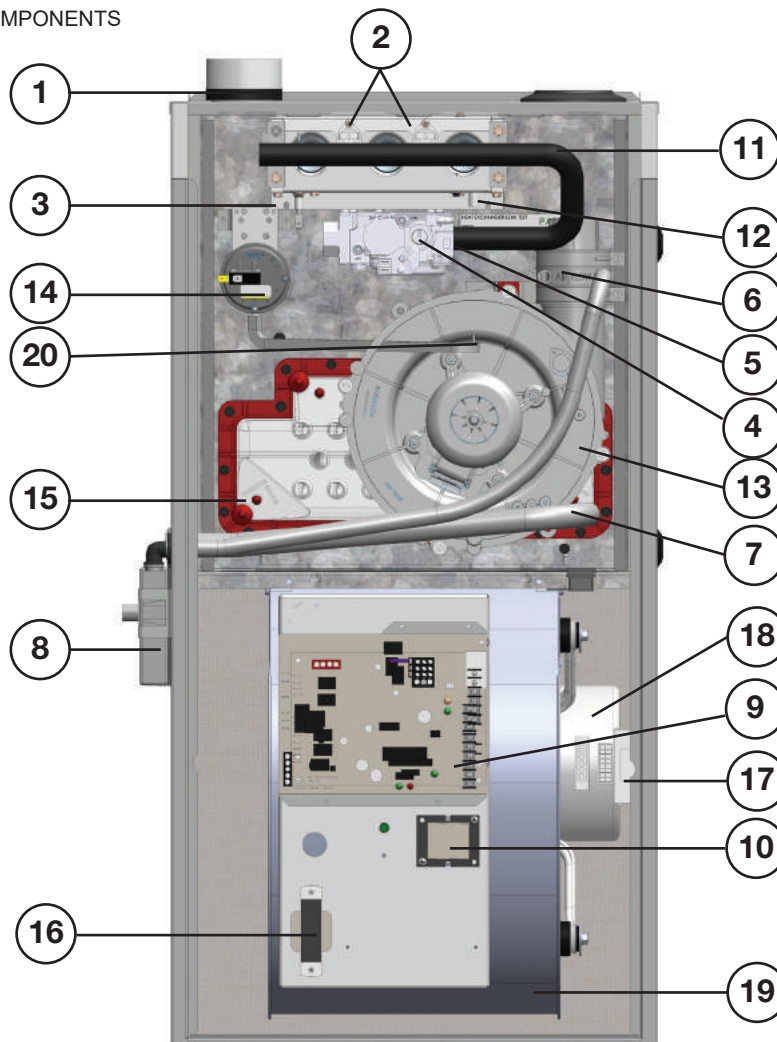
FIGURE 1 - FURNACE COMPONENTS
