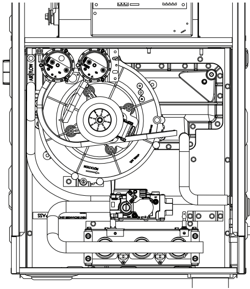
RIGHT VENT INSTALLATION - LEFT DRAIN (INTERNAL)
