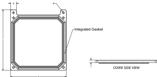
COVER BOTTOM VIEW
