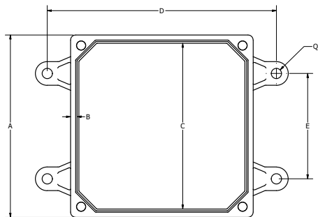
BOX TOP VIEW
