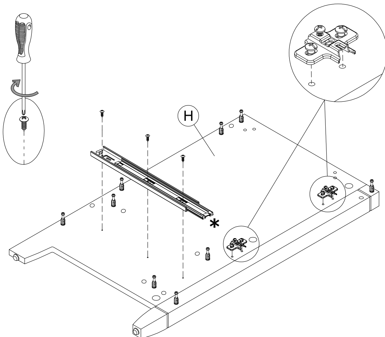
Mounting Plate
