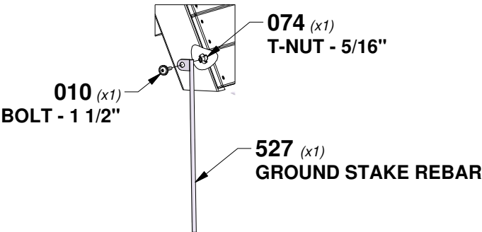
DETAIL 'D'
