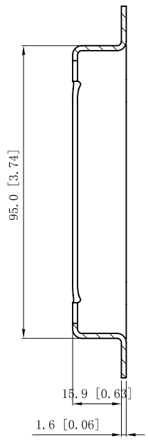
VIEW B-B
