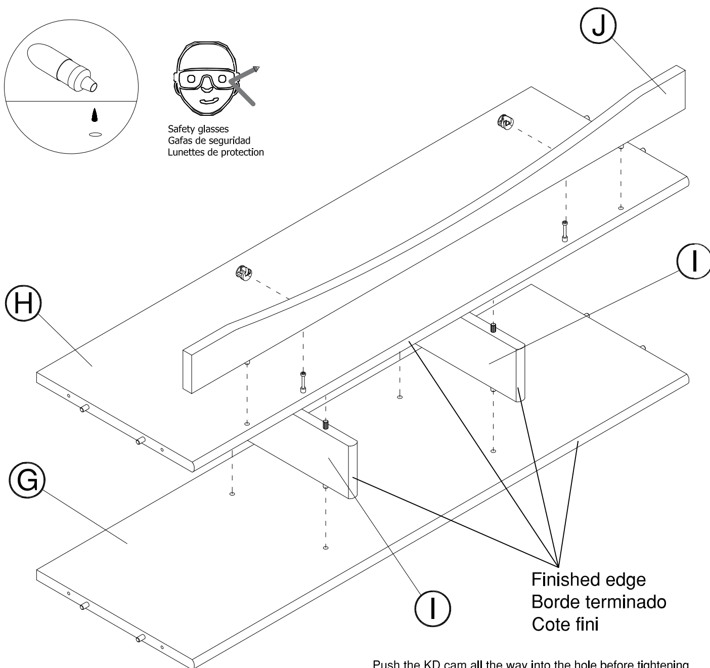
KD Cam
