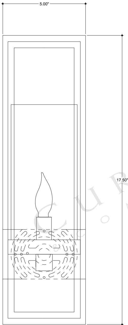
FRONT VIEW
