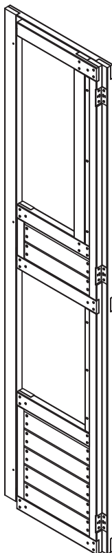
1pc. - [9264] - 63.5 x 558.8 x 2286mm 2-1/2 x 22 x 90" Folding Panel Assembly Left A - 37859264
