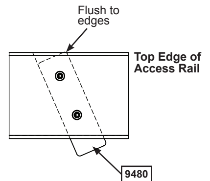
Fig. 17.3 End View
