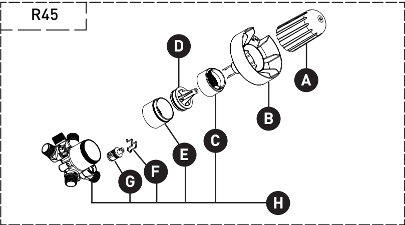
R45 3-way Type T/P Coaxial Valve Rough without Cartridge
