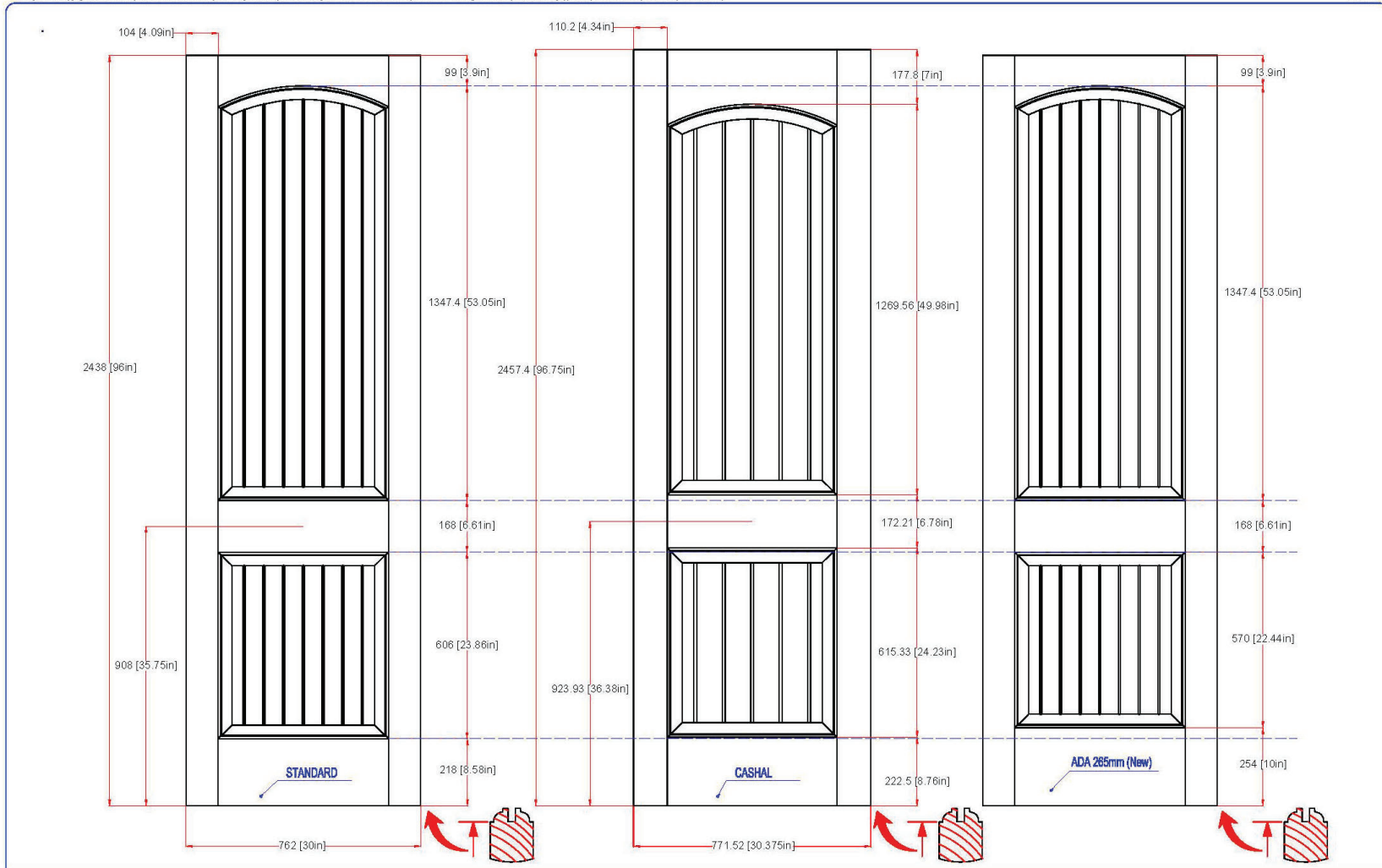
(Comparison STANDARD - CRAFTMASTER - ADA 265mm New) ARCH TOP PANEL 35 mm (1 3/8") (V GROOVED)
